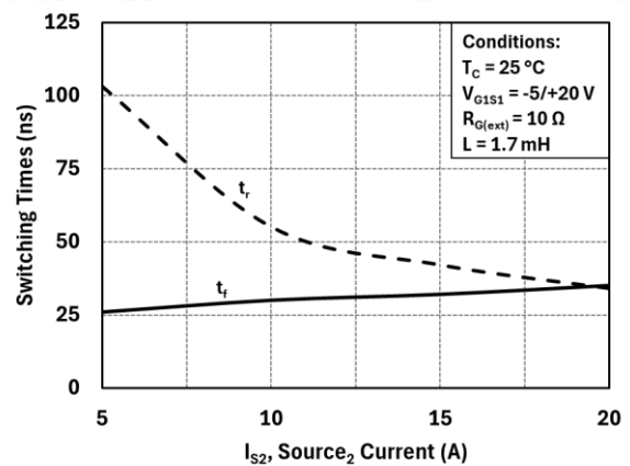
Figure 6: Switching Times Vs. Current
